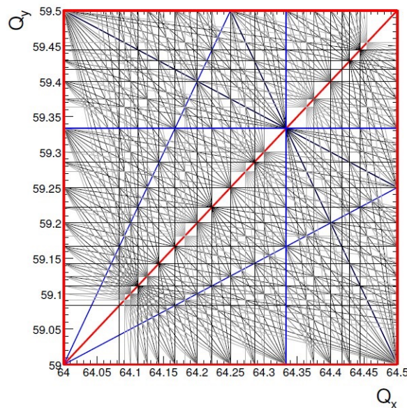
(a) Full tune diagram
