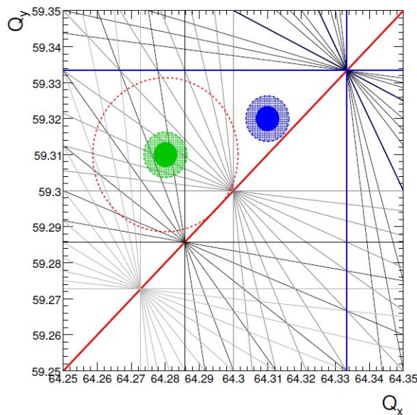
(b) Zoom around LHC Q working points
